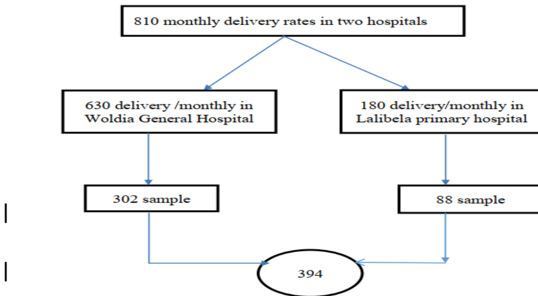
Figure 1: Sampling procedure
